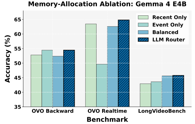
Figure 4 | Effect of query-adaptive memory allocation on Gemma 4 E4B. All policies use the same constructed memory and decoder-facing budget; only the allocation between recent and event memory differs.
