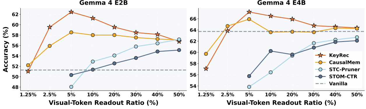
Figure 2 | Readout-budget scaling on StreamingBench. Results are shown for Gemma 4 E2B (left) and Gemma 4 E4B (right). Dashed horizontal lines denote uncompressed Vanilla performance. The horizontal axis reports the decoder-facing visual-token ratio. KeyRec selects each readout from a visual-token memory approximately twice as large, whereas each baseline decodes its complete retained token buffer (STOM-CTR: StreamingTOM-CTR).
