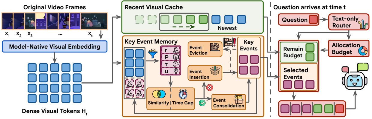
Figure 1 | Overview of KeyRec. During query-agnostic writing, incoming frames update a recent cache and a bounded key-event memory through event insertion, consolidation, and eviction. At query time, a text-only router allocates a fixed readout budget between recent and historical evidence for query-adaptive inference without replaying previous frames.
