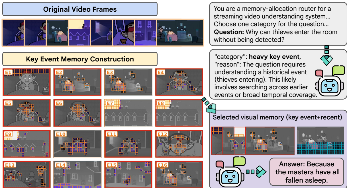
Figure 8 | KeyRec case study on StreamingBench with NEO-ov 2B. KeyRec constructs query-agnostic key events from selected visual patches, routes the history-dependent question to coverage-oriented retrieval, and produces a fixed-budget readout that supports the correct answer. The red border indicates the selected events after determining the budget allocation by the router.
