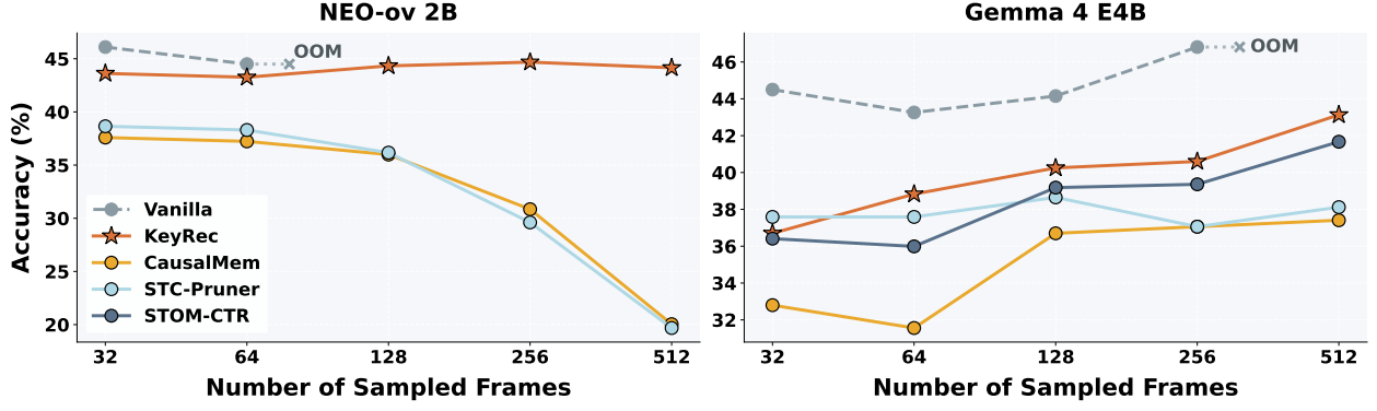
Figure 3 | Scaling with the number of sampled frames on LongVideoBench’s (900s, 3600s] duration group. All compressed methods use a 10% decoder-facing ratio. Missing Vanilla results indicate memory limitations; StreamingTOM-CTR (STOM-CTR) does not support NEO-ov.
