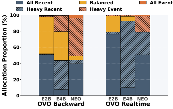
Figure 6 | Router-state distributions across backbones on OVO-Bench. Each stacked bar shows the percentage of questions assigned to each state. Across backbones, realtime questions favor recent memory, while backward questions shift toward balanced or event-oriented ones.
